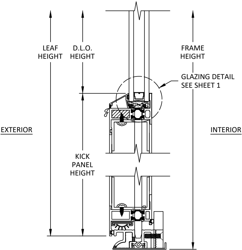
C 5 VERTICAL SECTION SILL W/ KICK PANEL
