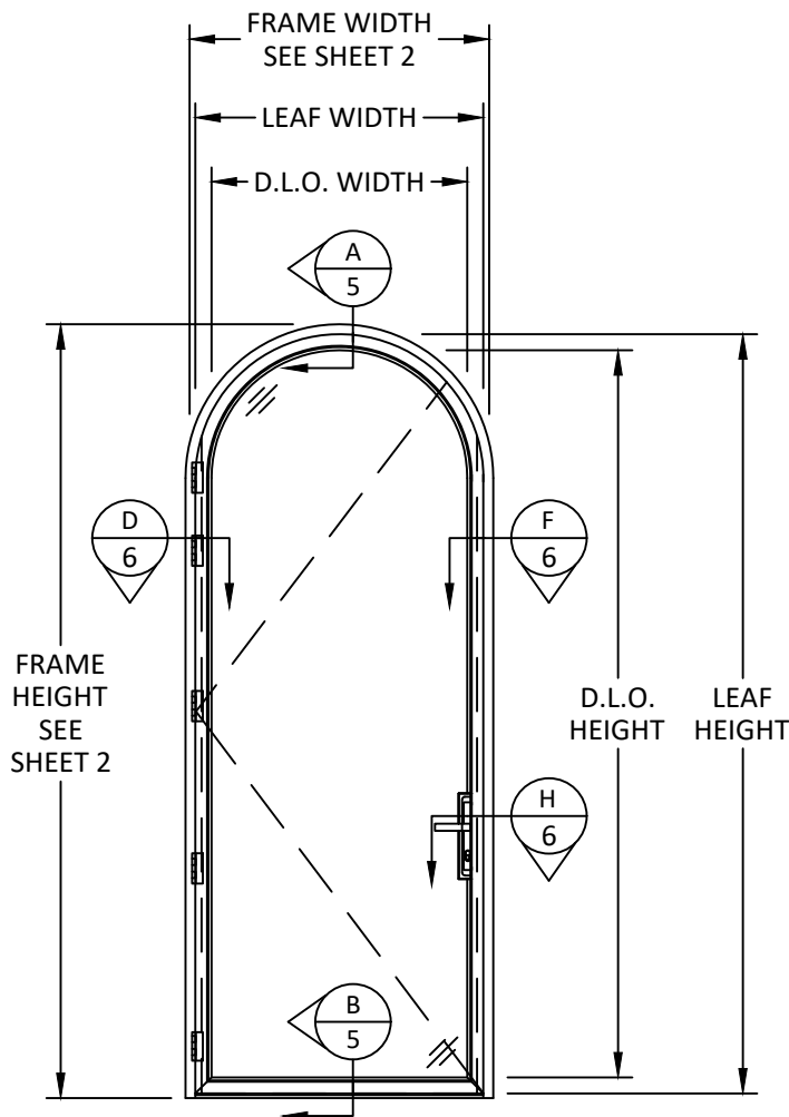
TYPICAL ELEVATION SINGLE DOOR, ROUND TOP
