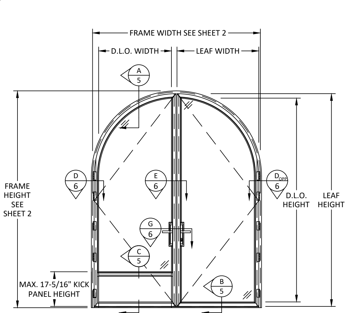
TYPICAL ELEVATION FRENCH DOOR, ROUND TOP
