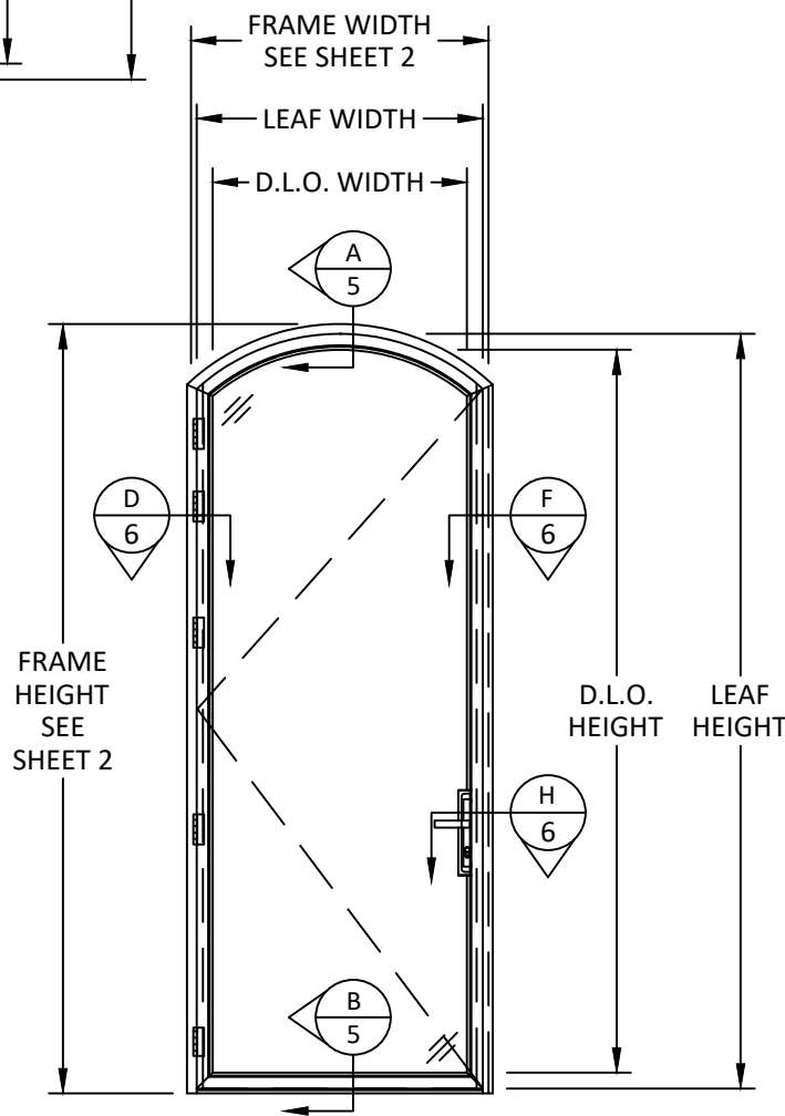
TYPICAL ELEVATION SINGLE DOOR, ARCH TOP
