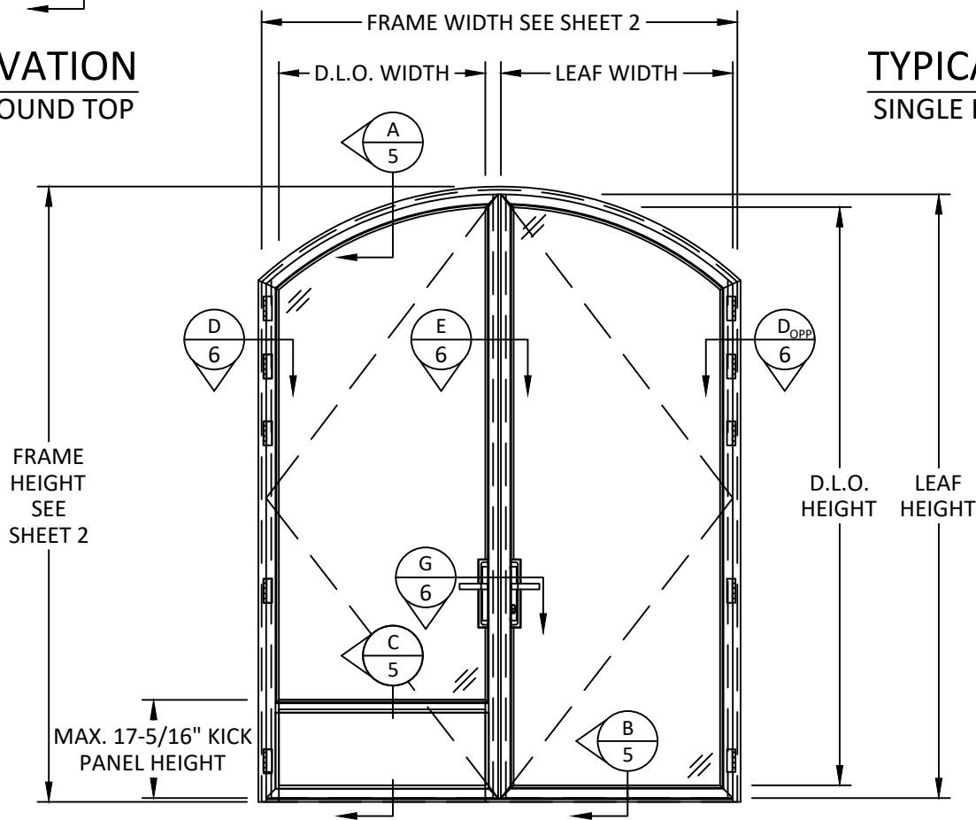
TYPICAL ELEVATION FRENCH DOOR, ARCH TOP
